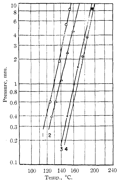
Fig. 1.—Boiling points of \text{CH}_3\text{COOCH}(\text{CH}_3)\text{COOCH}(\text{CH}_3)\text{COOR} : 1, R is -\text{CH}_2\text{CH}_2\text{O}(\text{CH}_2)_4\text{H} ; 2, R is -\text{CH}_2\text{CH}(\text{O})\text{CH}_2\text{CH}_2\text{CH}_2 ; 3, R is -\text{CH}_2\text{CH}_2\text{OCH}_2\text{CH}_2\text{Cl} ; 4, R is -\text{CH}_2\text{CH}_2\text{OCH}_2\text{CH}_2\text{O}(\text{CH}_2)_4\text{H} .
